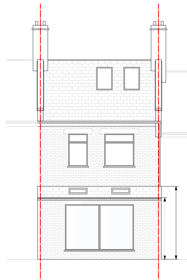
REAR ELEVATION
